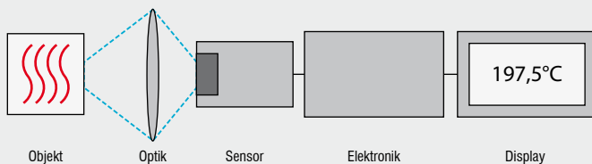
Infrarot System
