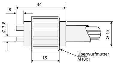
CFS: FA-Adapter System FASOP
